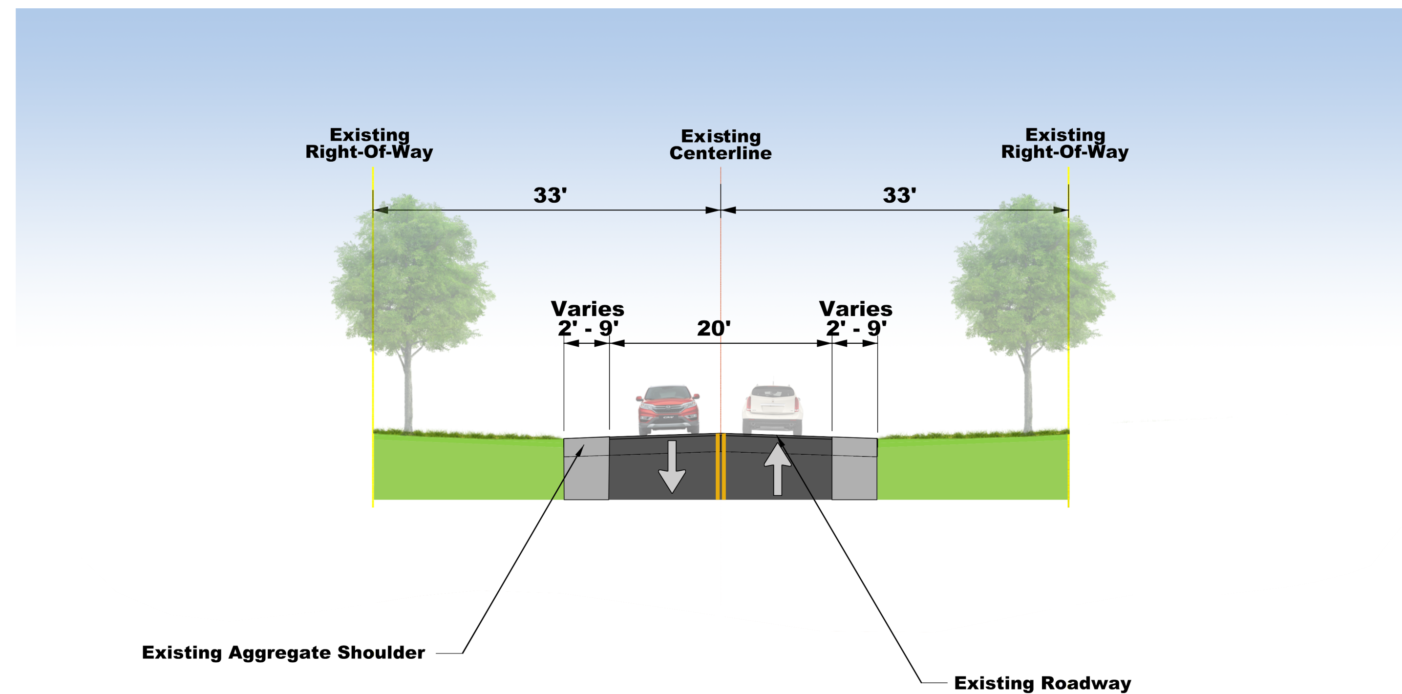
EXISTING TYPICAL SECTION
