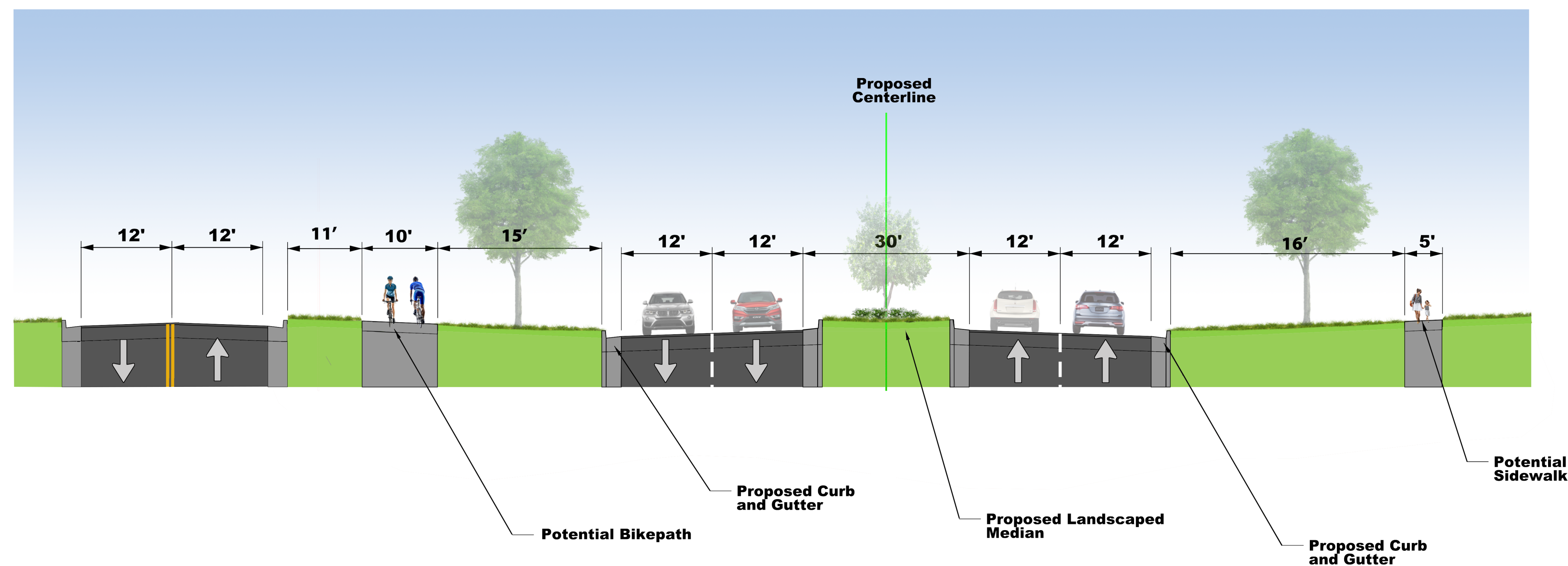
PROPOSED TYPICAL SECTION
